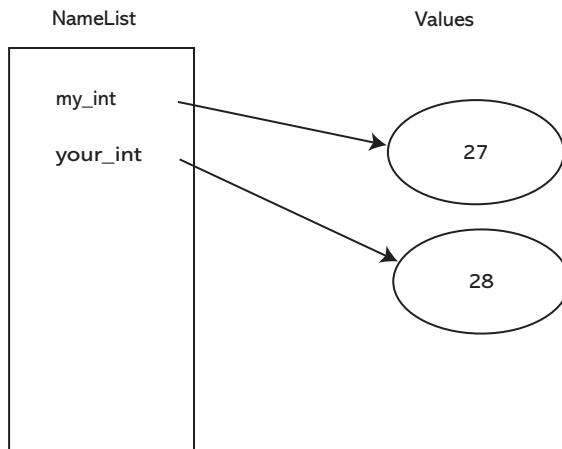
FIGURE 7.3 Modification of a reference to an immutable object.
