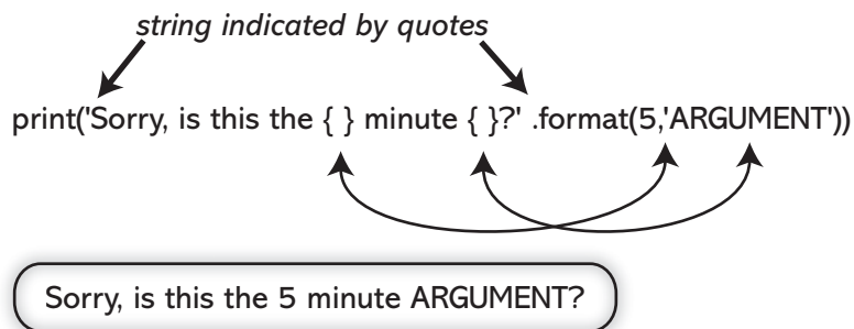
FIGURE 4.10 String formatting example.
