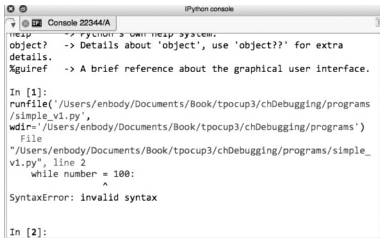
FIGURE C.5 Syntax error flagged in the shell. [Screenshot from Python. Copyright © by Python. Used by permission of Python.]
