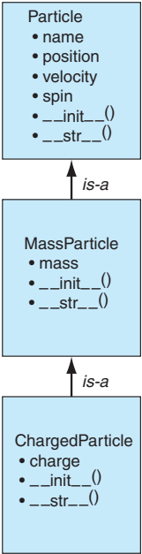
FIGURE 12.4 The particle class hierarchy.
