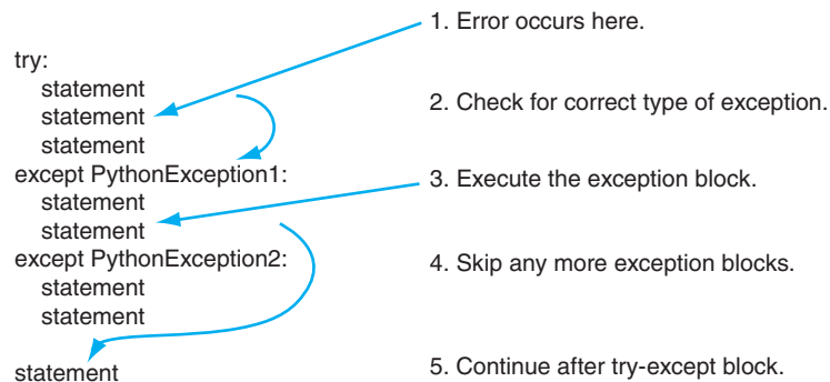
FIGURE 14.5 Exception flow.
