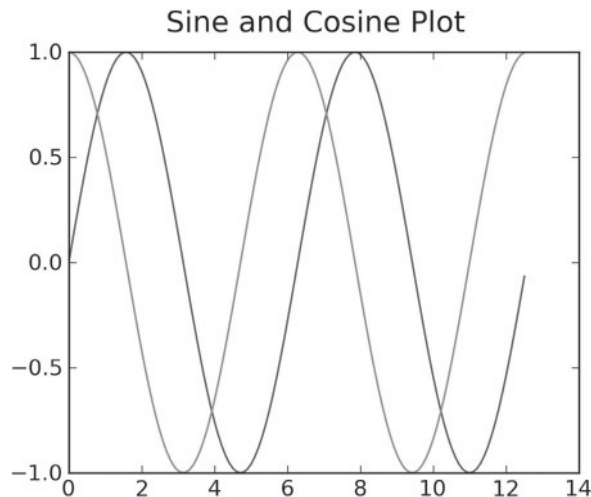
FIGURE 7.14 A graph of sine and cosine from 0 to about 4\pi .
