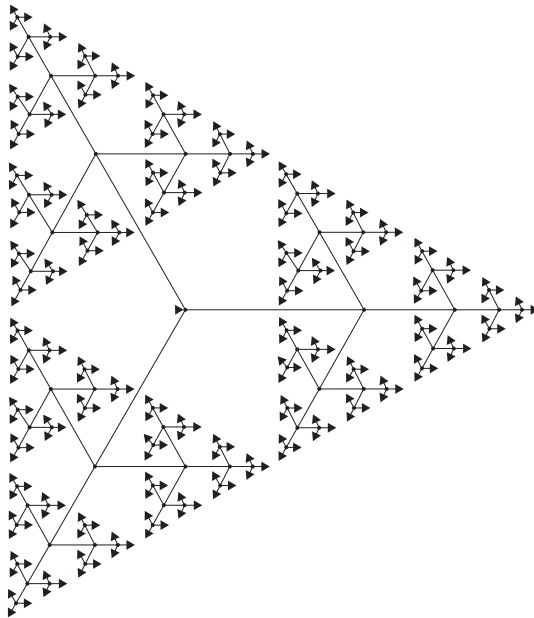
FIGURE 15.6 Sierpinski triangle.
