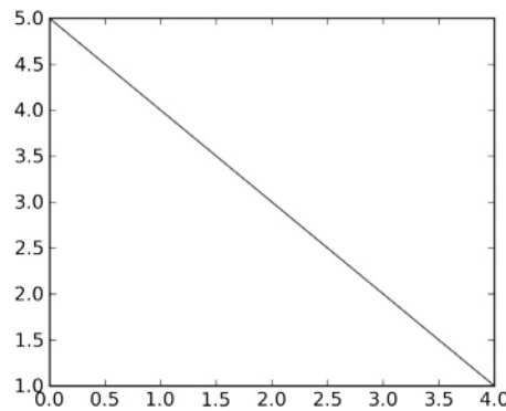
FIGURE D.1 First plot
