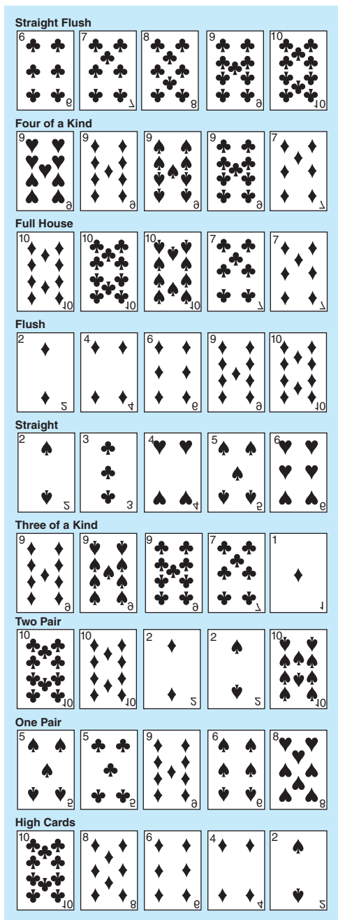
FIGURE 6.2 Poker hand rankings.
