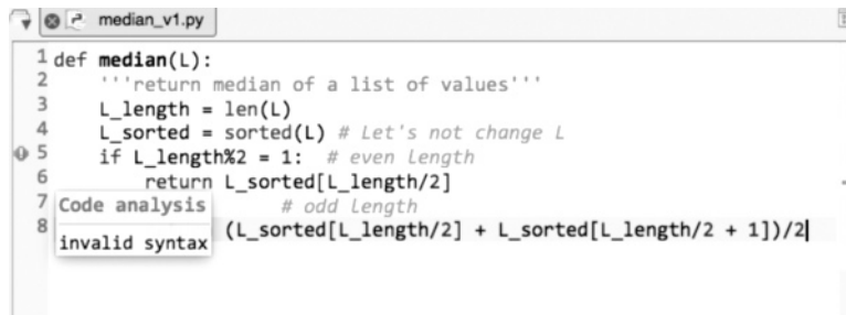
FIGURE C.10 Flagged syntax error. [Screenshot from Python. Copyright © by Python. Used by permission of Python.]
