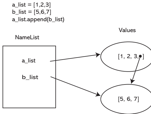
FIGURE 7.9 Lists after append.
