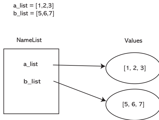
FIGURE 7.8 Simple lists before append.
