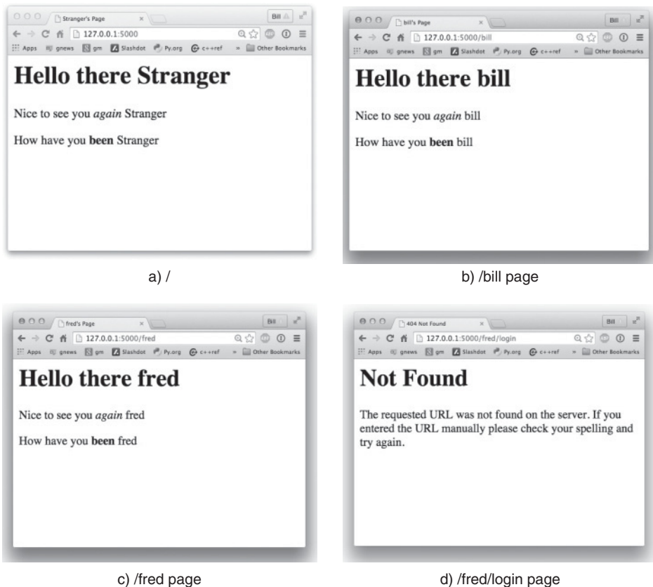
FIGURE E.6 Passing web address to our display function. [William F. Punch, Richard J. Enbody.]
