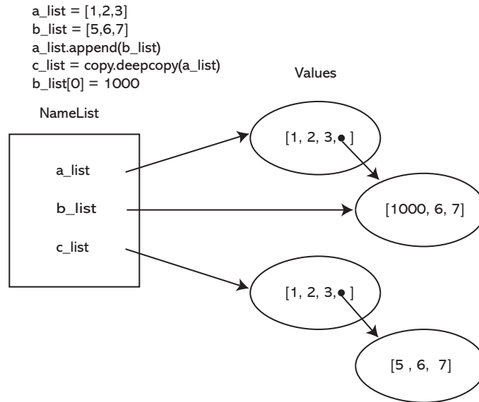
FIGURE 7.12 Using the copy module for a deep copy.
