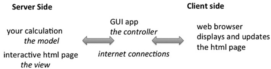
FIGURE E.1 MVC: Model-View-Controller.
