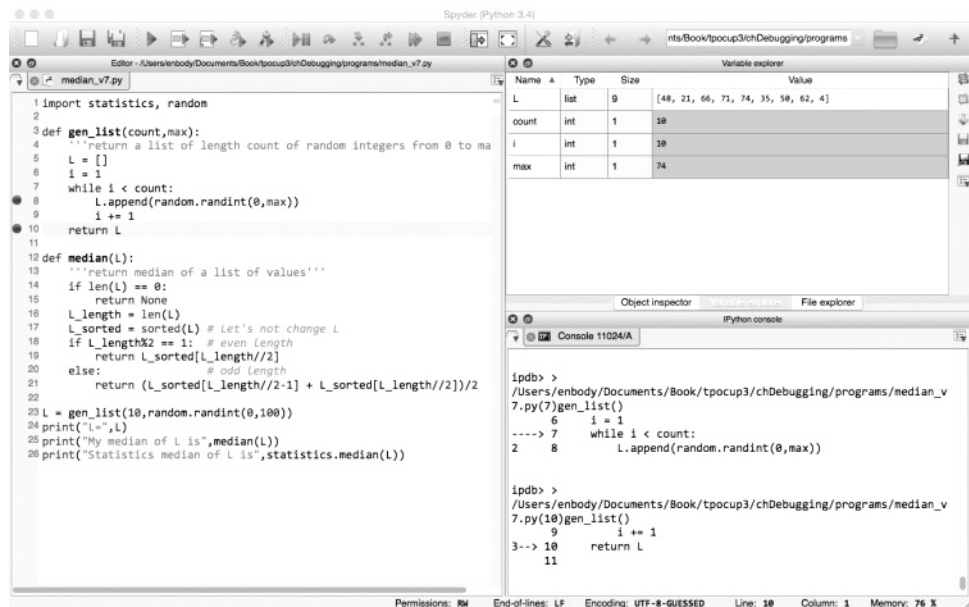
FIGURE C.15 Two breakpoints. [Screenshot from Python. Copyright © by Python. Used by permission of Python.]
