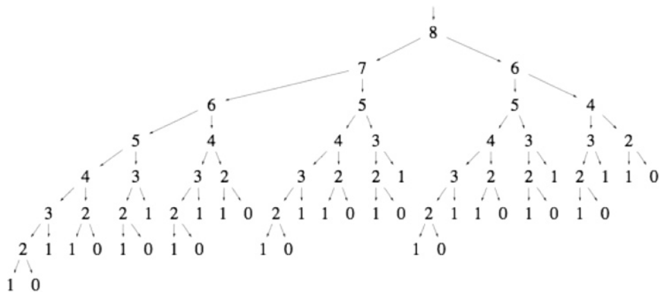
FIGURE 15.4 The simple Fibonacci code recalculates the same value.
