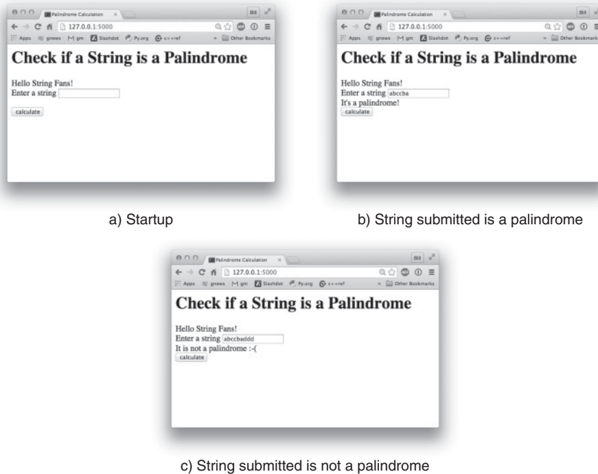
FIGURE 4.13 The Palindrome GUI Example. [William F. Punch, Richard J. Enbody.]
