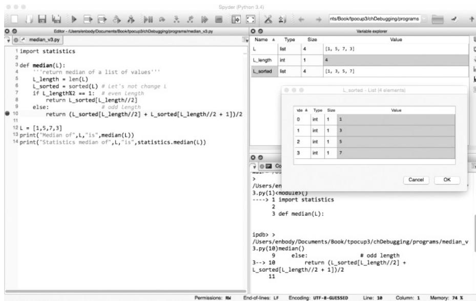
FIGURE C.13 Collection pop-up in Variable Explorer. [Screenshot from Python. Copyright © by Python. Used by permission of Python.]
