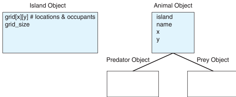
FIGURE 13.1 Objects: island, animals, predators, and prey.
