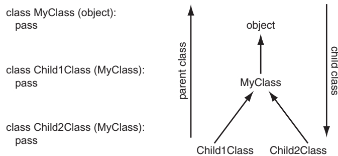
FIGURE 12.1 A simple class hierarchy
