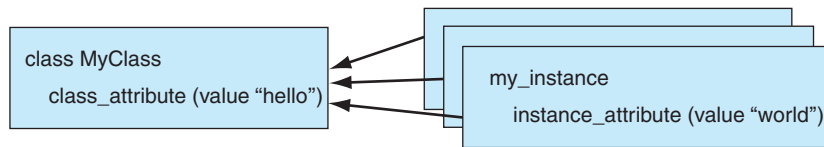
FIGURE 11.3 The instance-of relationship.
