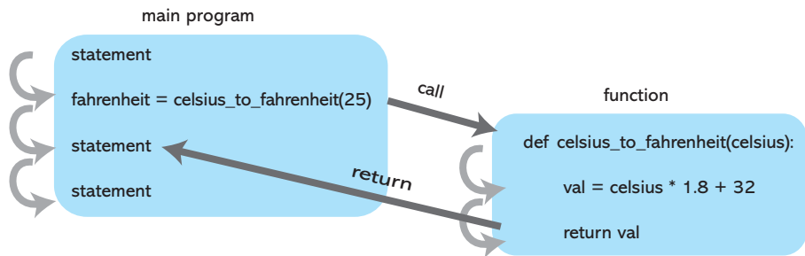
FIGURE 5.2 Function flow of control.
