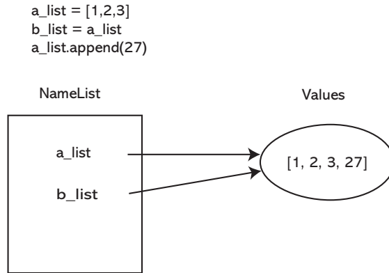
FIGURE 7.5 Modification of shared, mutable objects.
