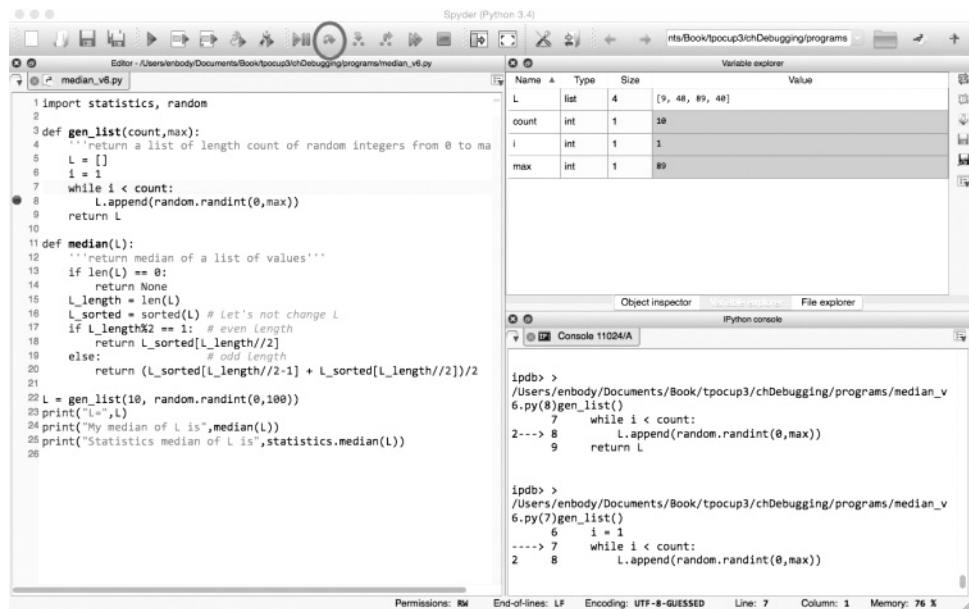
FIGURE C.14 Stepping one line at a time in the debugger. [Screenshot from Python. Copyright © by Python. Used by permission of Python.]
