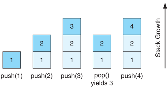
FIGURE 15.2 The operation of a stack data structure.
