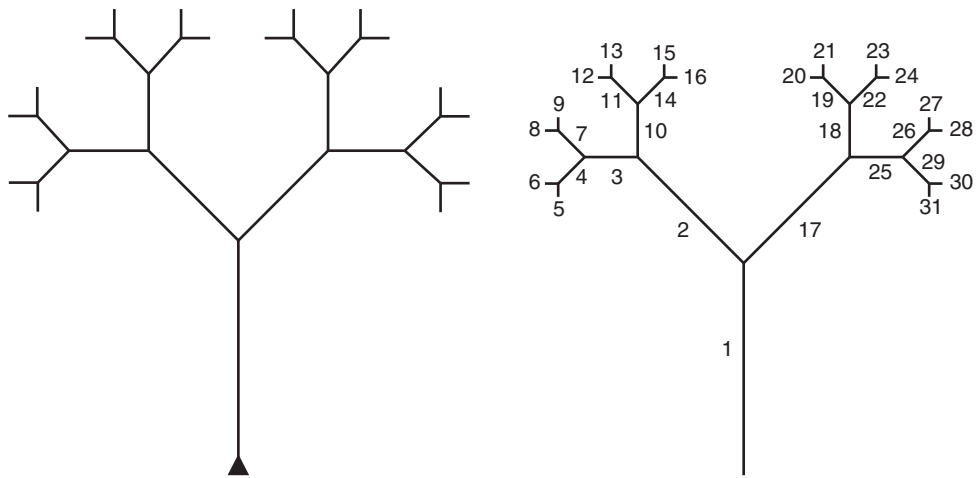
FIGURE 15.5 Recursive tree: (a) Python-drawn on left; (b) order-of-drawing on right.
