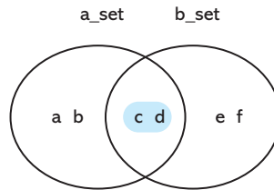
FIGURE 9.3 Intersection of {'a', 'b', 'c', 'd'} and {'c', 'd', 'e', 'f'}.
