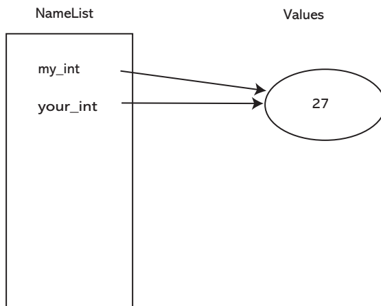
FIGURE 7.2 Namespace snapshot #1.
