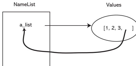
FIGURE 7.7 Self-referencing.
