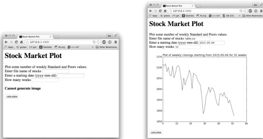
FIGURE 10.7 S&P Plot. [William F. Punch, Richard J. Enbody.]
