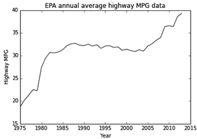
FIGURE 7.13 Plot of EPA highway mileage from 1975.
