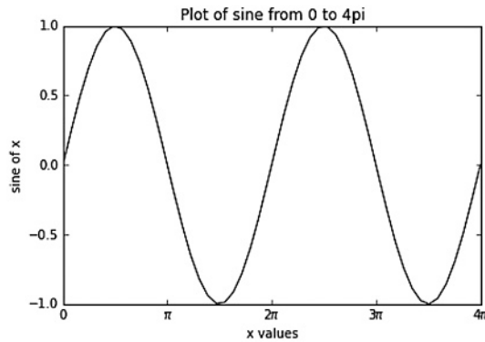
FIGURE D.3 Sine with improved labels.
