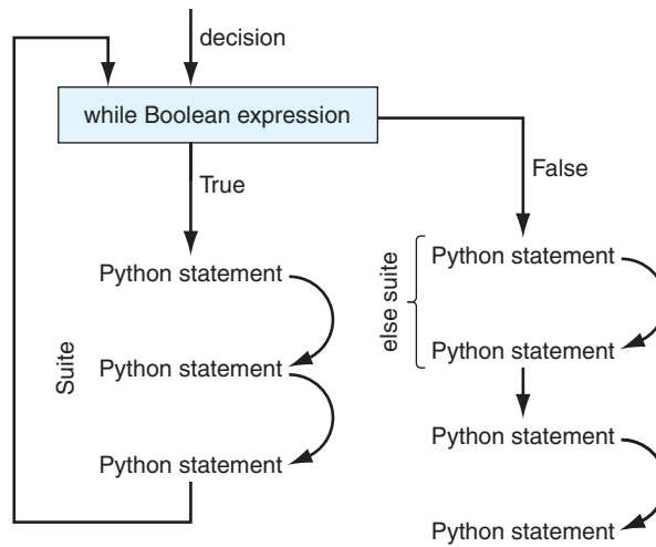
FIGURE 2.9 while-else .
