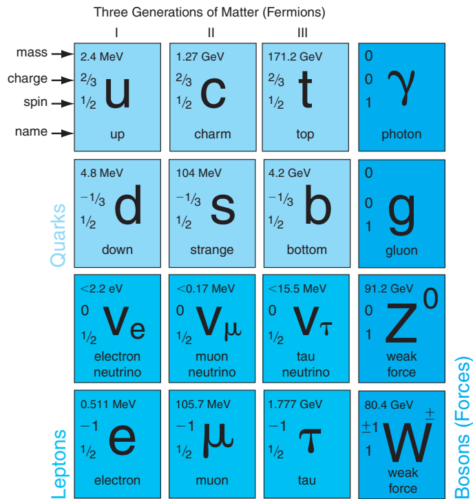
FIGURE 12.3 The Standard Model of physics.
