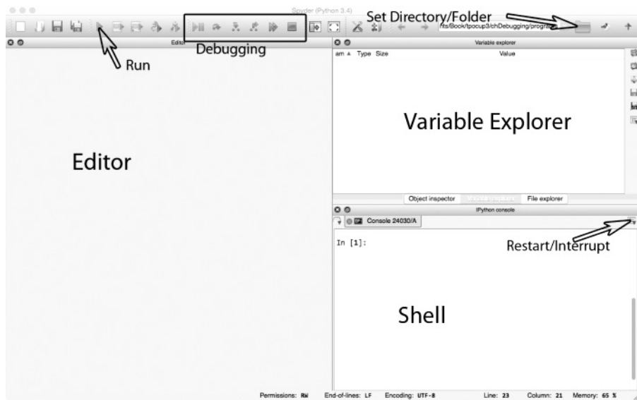
FIGURE A.5 Anaconda's Spyder IDE. [Screenshot from Python. Copyright © by Python. Used by permission of Python.]
