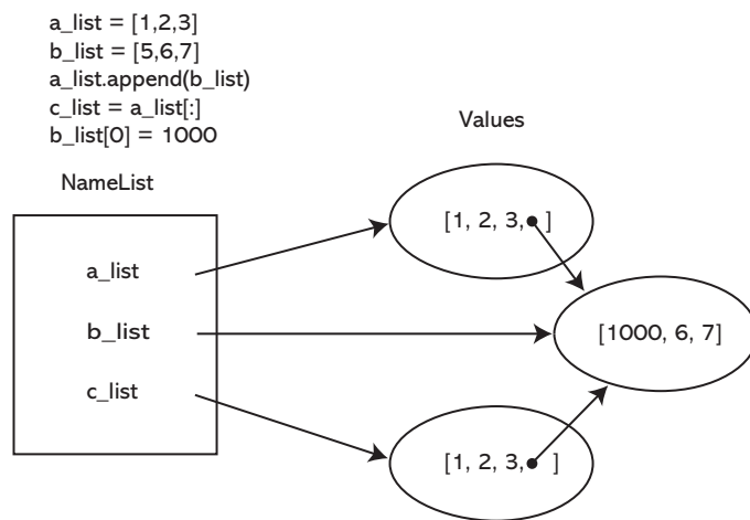
FIGURE 7.11 Effects of copy slice (a shallow copy).
