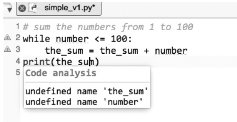
FIGURE C.6 Undefined name error. [Screenshot from Python. Copyright © by Python. Used by permission of Python.]
