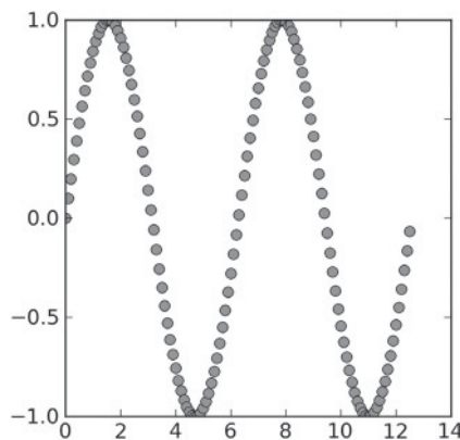
FIGURE 2.11 Sine plot with matplotlib.
