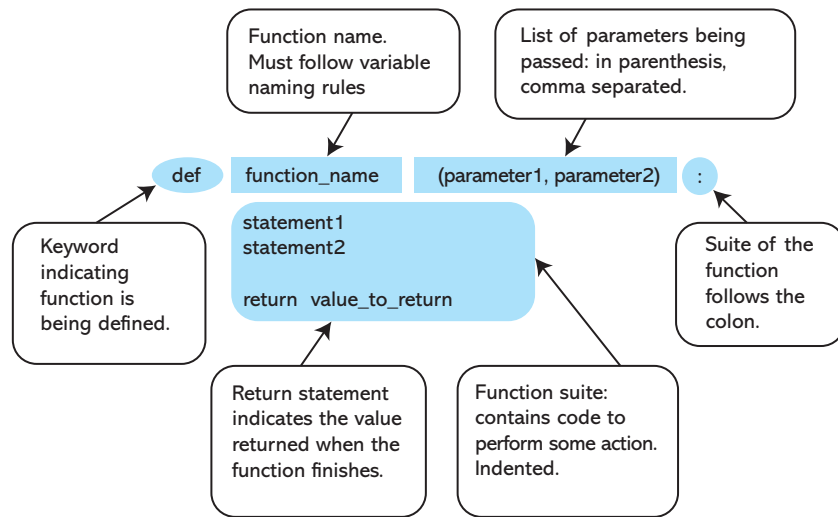
FIGURE 5.1 Function parts.
