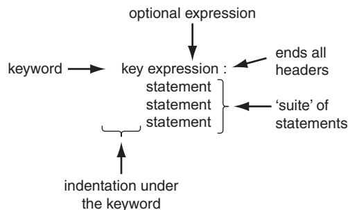
FIGURE 2.3 Control expression.
