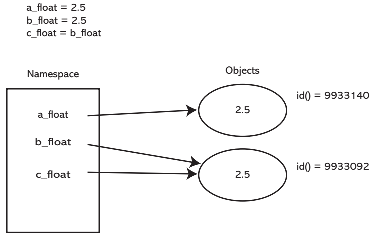
FIGURE 2.6 What is equality?
