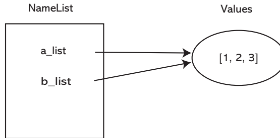
FIGURE 7.4 Namespace snapshot after assigning mutable objects.
