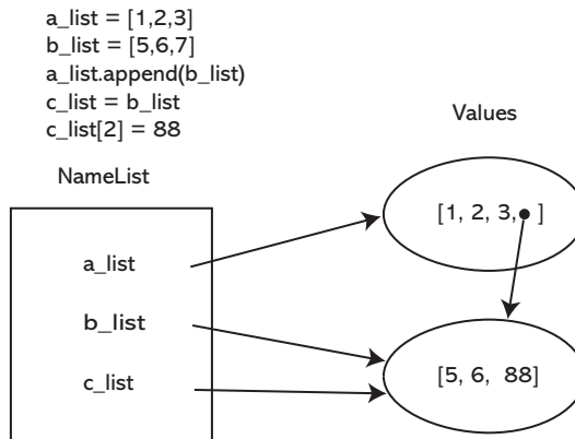
FIGURE 7.10 Final state of copying example.
