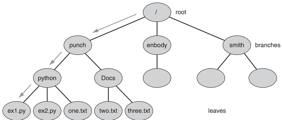
FIGURE 14.4 Directory tree with path /punch/python/ex1.py highlighted.
